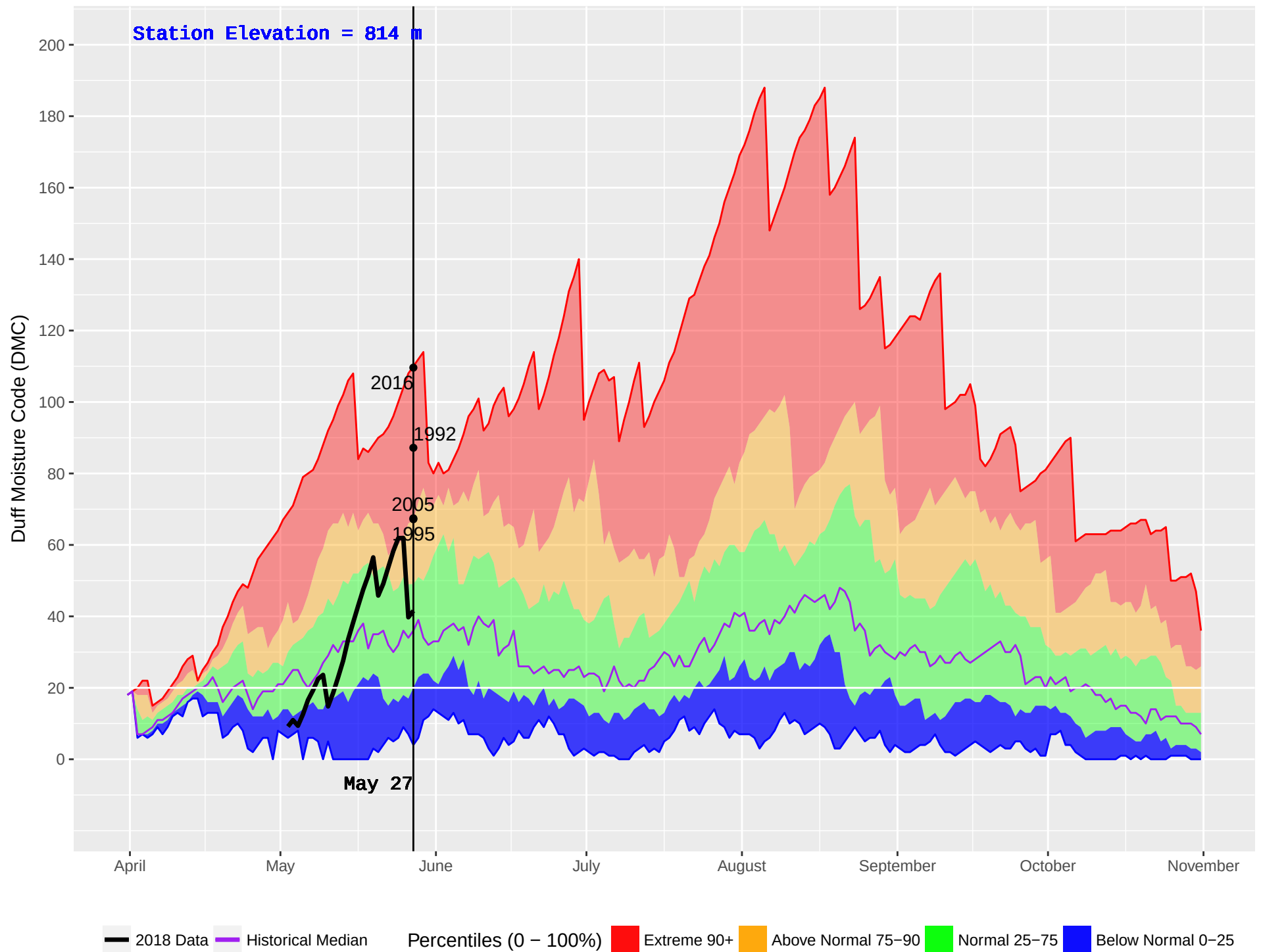
CHILAKO (189) : Historical (1986–2016) and Current (2018) Noon Duff Moisture Code (DMC)
