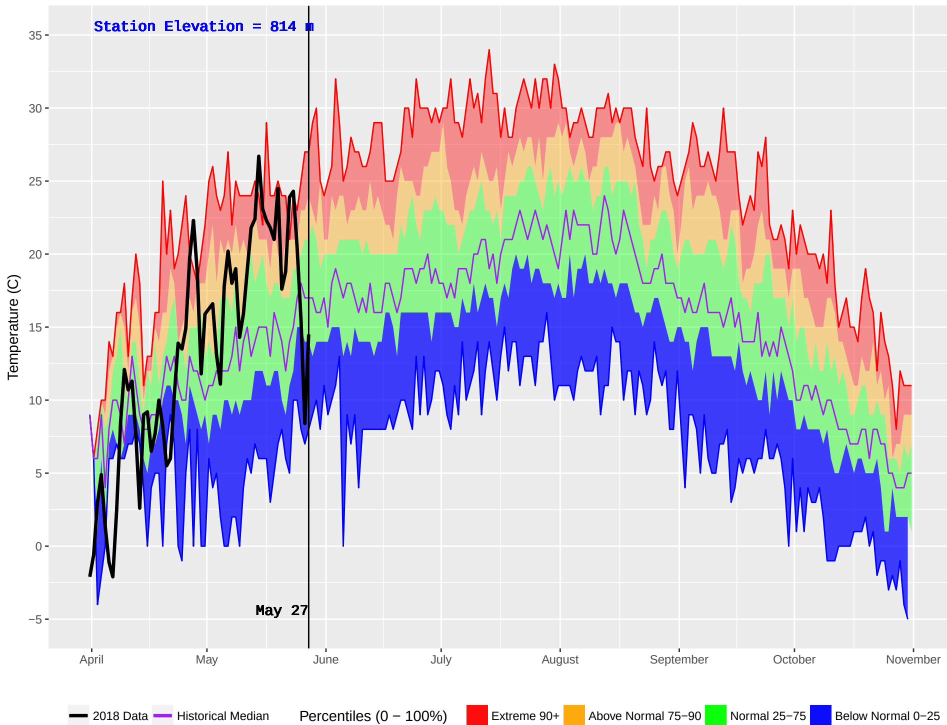
CHILAKO (189) : Historical (1986–2016) and Current (2018) Noon Temperature
